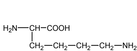
lysine
